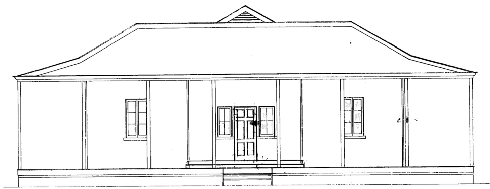
Back Elevation S.E.
