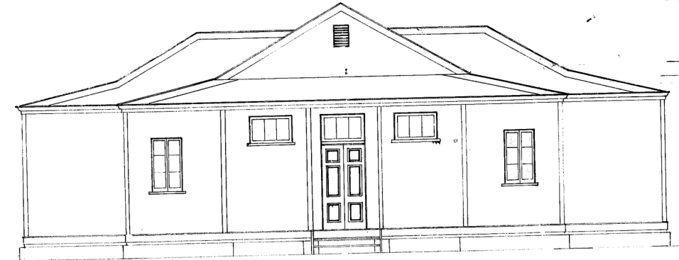
Front Elevation.N.W. Scale of Feet
